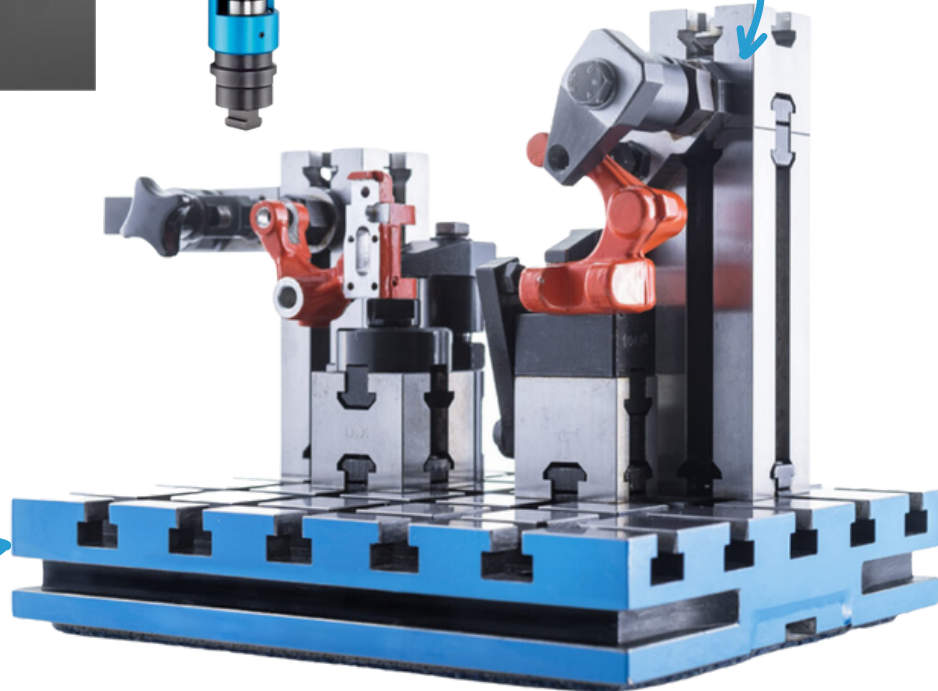
FLOATING CLAMPS
