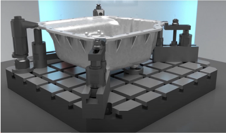
SUPPORTING ELEMENTS
